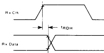
FIGURE 5 — RECEIVE DATA HOLD TIME (+ 1 Mode)
